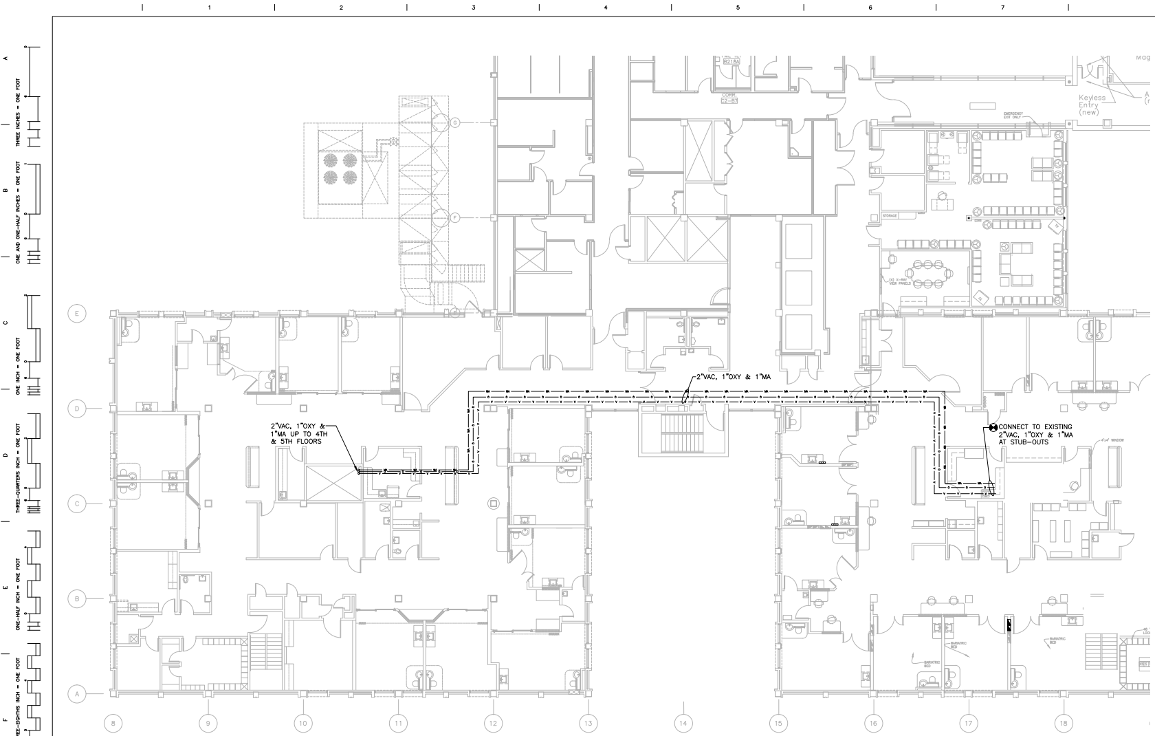
SECOND FLOOR WARD EAST MEDICAL GAS PLAN SCALE: 1/8" = 1'-0"
