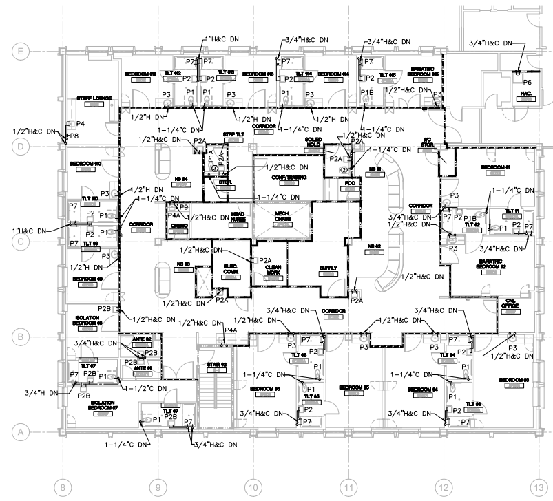
FIFTH FLOOR WARD EAST HOT AND COLD WATER PLAN SCALE: 1/8" = 1'-0"
