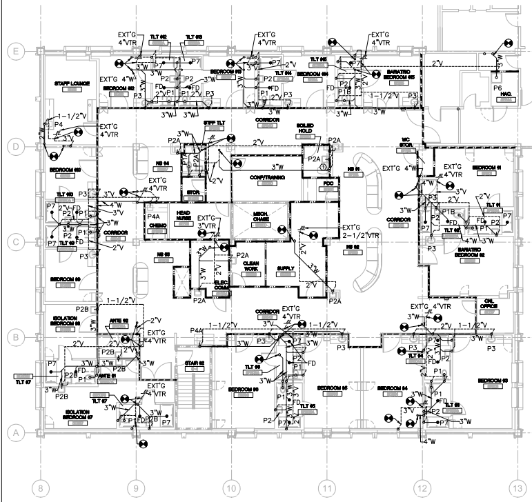
FIFTH FLOOR WARD EAST WASTE AND VENT PLAN SCALE: 1/8" = 1'-0"
