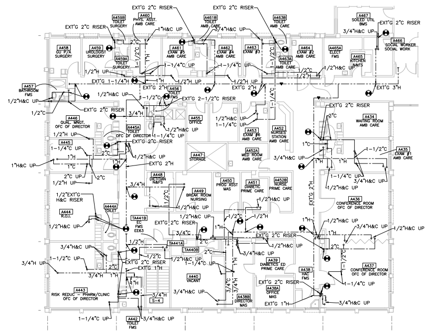
FOURTH FLOOR WARD EAST HOT AND COLD WATER PLAN SCALE: 1/8" = 1'-0"
