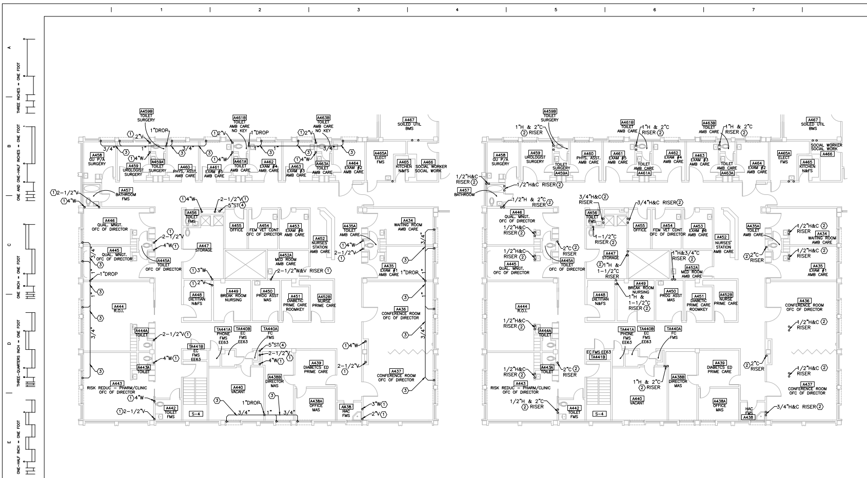
FOURTH FLOOR WARD EAST WASTE AND VENT DEMOLITION PLAN SCALE: 1/8" = 1' - 0"
