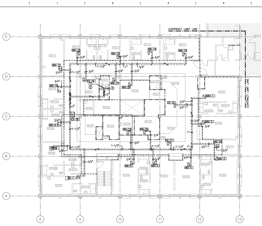
FIFTH FLOOR MECHANICAL PIPING PLAN SCALE: 1/8" = 1'-0"
